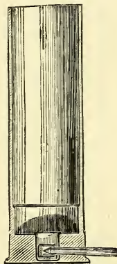
Section of the Lefauchaux Pin-fire Cartridge Case.
